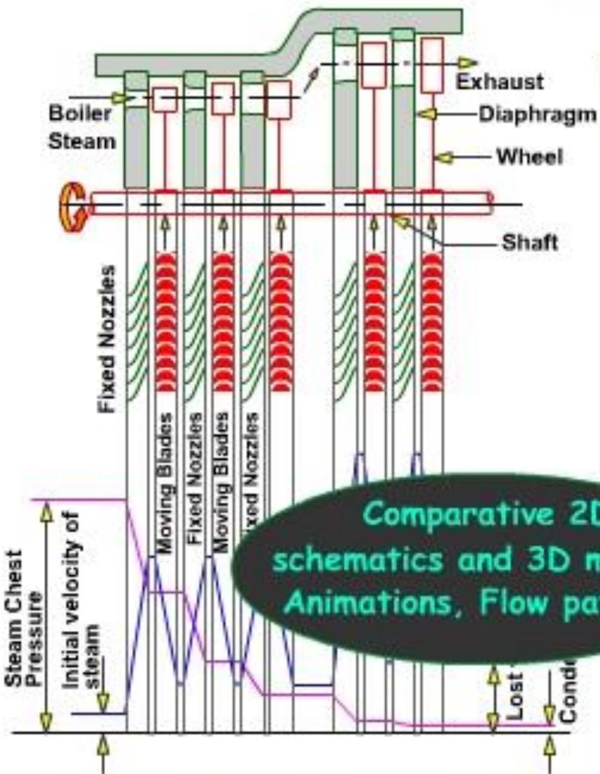
Diagrammatic Arrangement of Pressure-compounded Impulse Turbine
