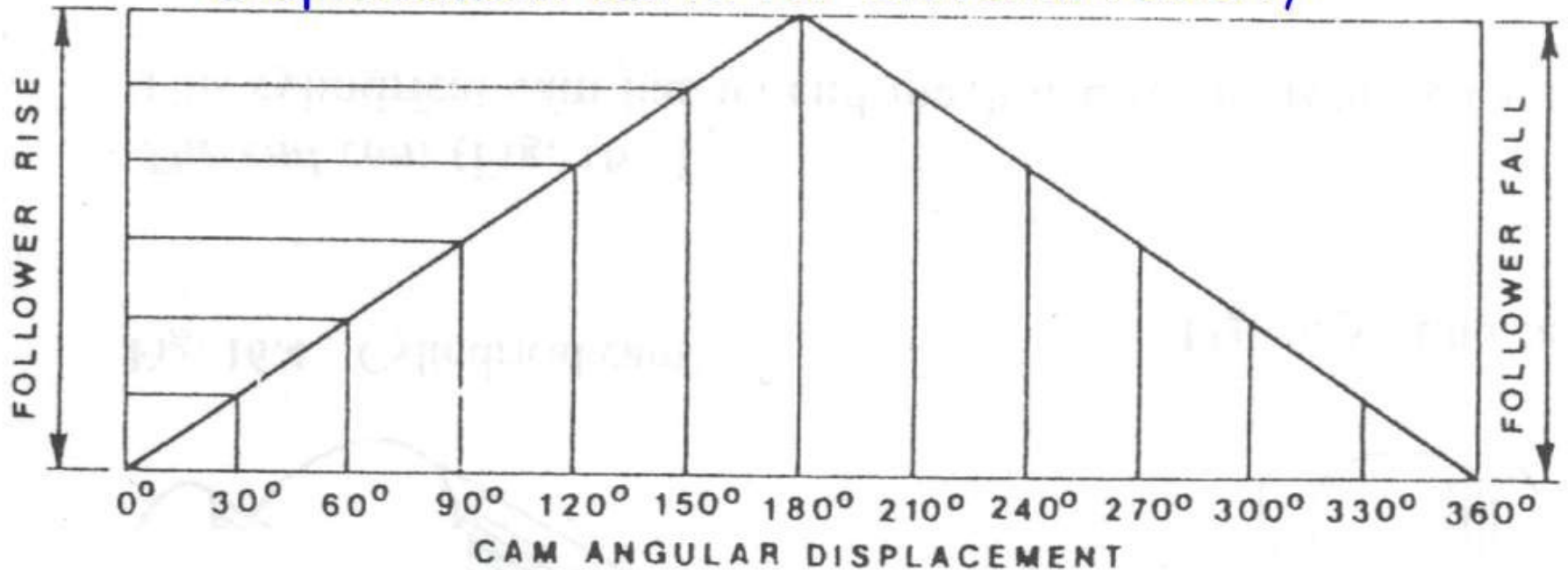
Displacement curve for Uniform velocity
