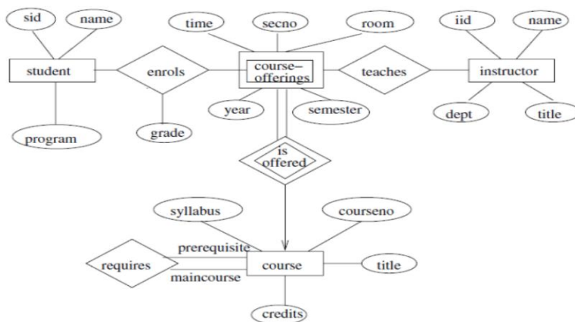
E-R diagram for a university.
