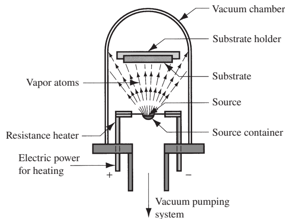
■ Figure U5.4 Setup for vacuum evaporation physical vapor deposition.
