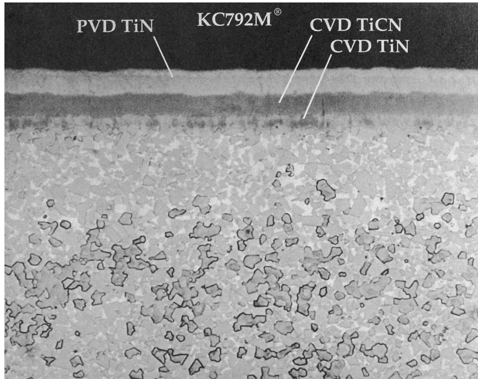
■ Figure U5.6 Photomicrograph of the cross section of a coated carbide cutting tool (Kennametal Grade KC792M); chemical vapor deposition was used to coat TiN and TiCN onto the surface of a WC-Co substrate, followed by a TiN coating applied by physical vapor deposition.
