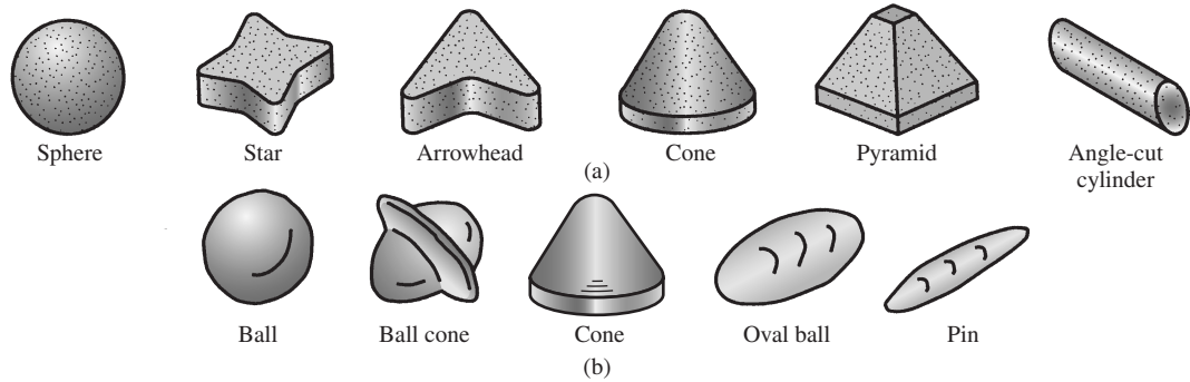
■ Figure U5.2 Typical preformed media shapes used in mass finishing operations: (a) abrasive media for finishing and (b) steel media for burnishing.
