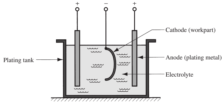
■ Figure U5.3 Setup for electroplating.
