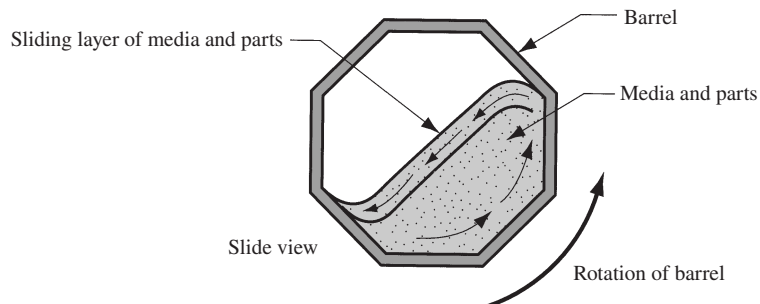
■ Figure U5.1 Diagram of tumbling (barrel finishing) operation showing “landslide” action of parts and abrasive media to finish the parts.
