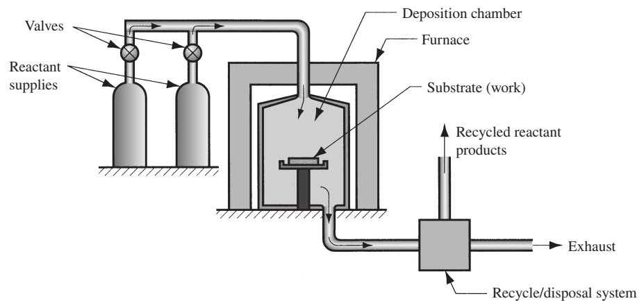
■ Figure U5.7 A typical reactor used in chemical vapor deposition.
