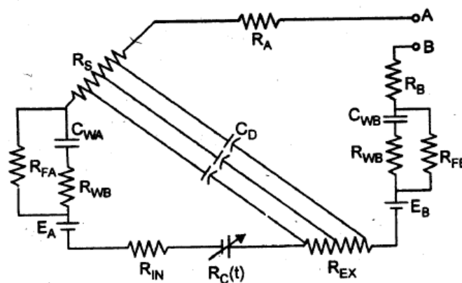
Figure 2.3 Equivalent Circuit
