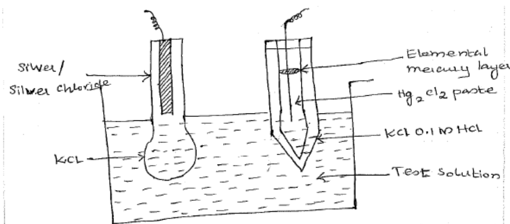
Figure 4.1 pH Electrode
