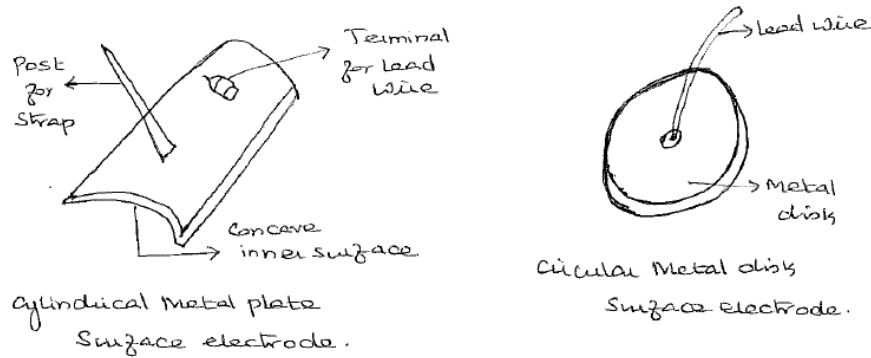
Figure 2.9 Surface Electrode
