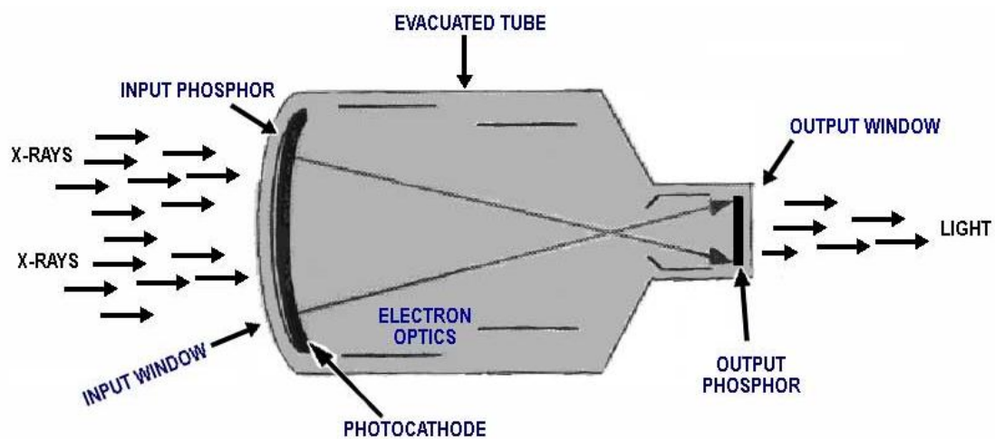
Figure 3.11 Image Intensifiers (Fluoroscopy)
