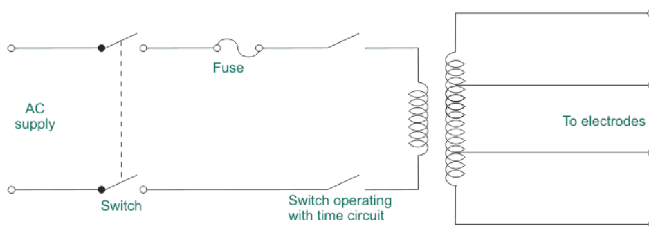
Figure 3.21 AC Defibrillator
