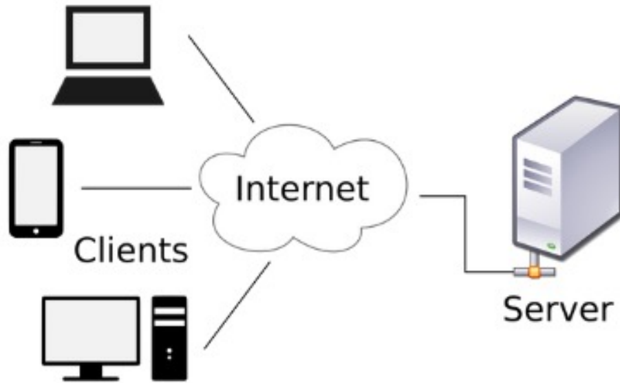
Client-Server
