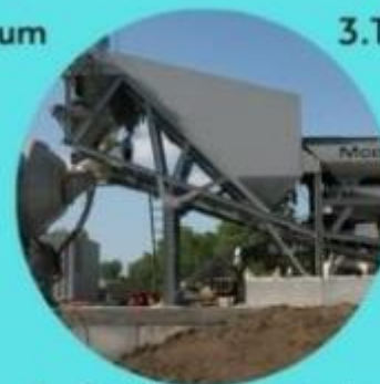
5. Continuous concrete mixers
