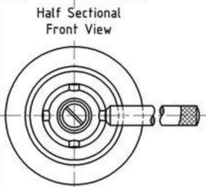
ASSEMBLY DRAWING OF SCREW JACK
