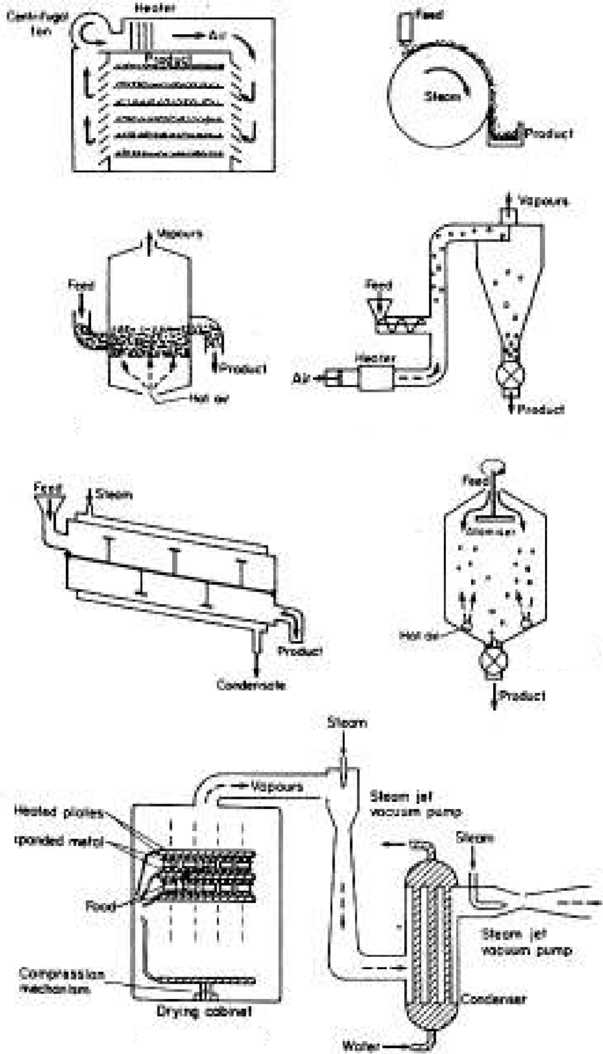
Figure 7.3 Dryers
