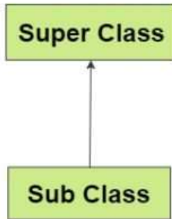
Single Inheritance
