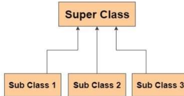
Hierarchial Inheritance
