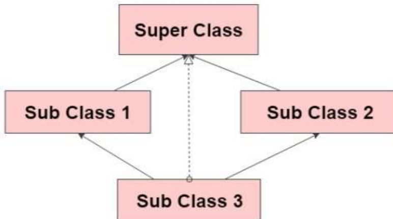
Hybrid Inheritance
