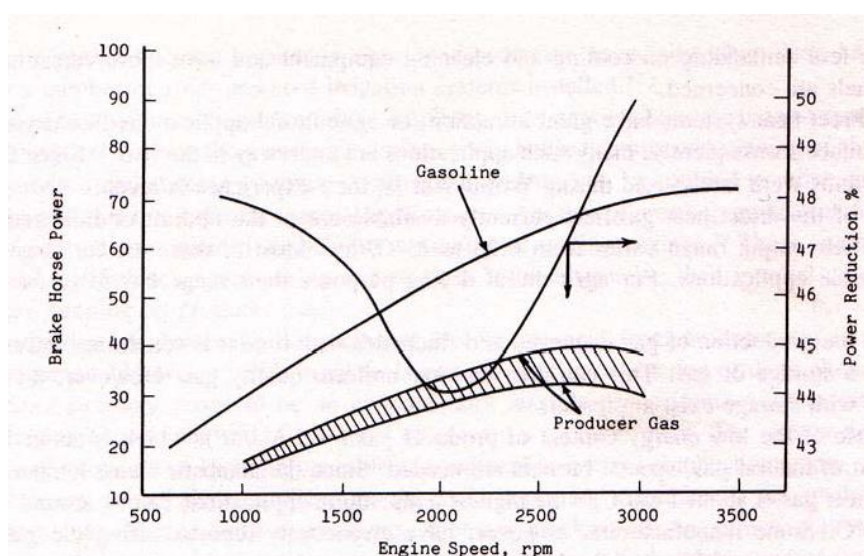
FIGURE 9. Power reduction as function of engine speed. (From Kaupp, A. and Goss, J. R., Small Scale Gas Producer Engine Systems , Deutsche Gesellschaft für Technische Zusammenarbeit, 1984. With permission.)
