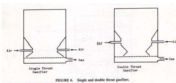
FIGURE 6. Single and double throat gasifiers.
