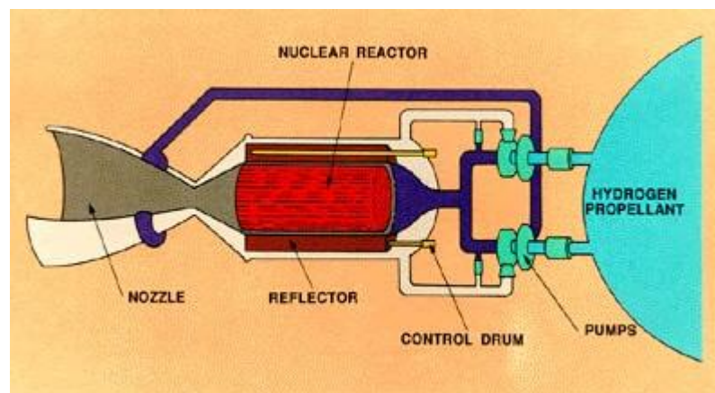
Solid Core Nuclear Rocket
