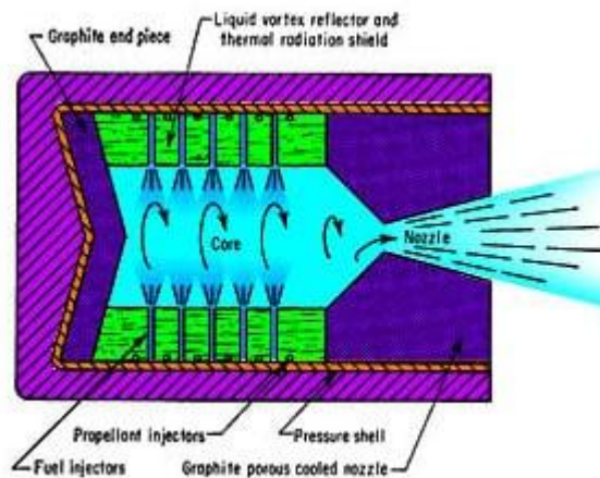
Liquid Core Nuclear Rocket
