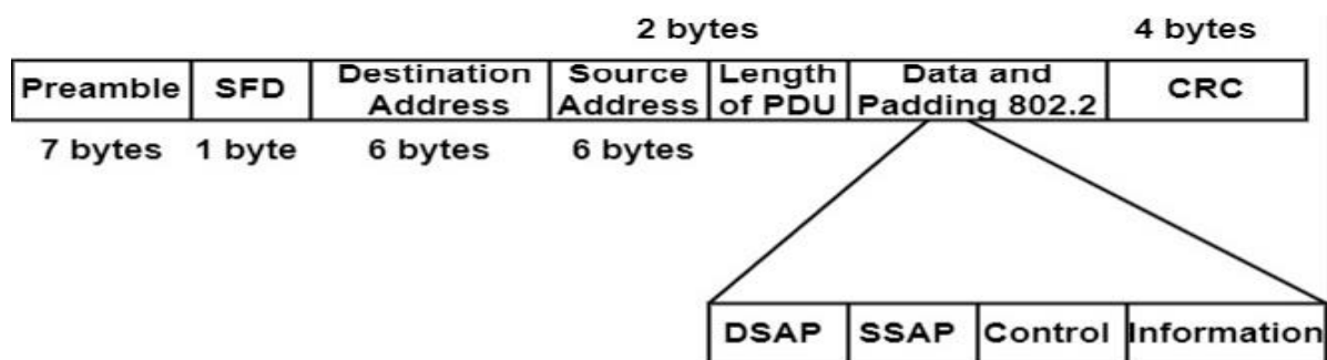
802.3 MAC Frame
