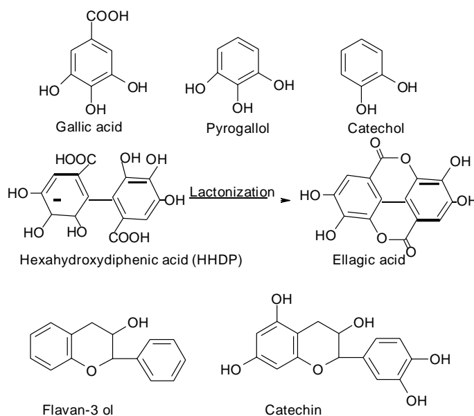
Fig.8. Precursors of tannins
