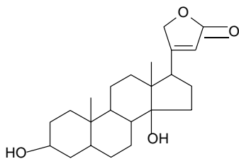
Fig. 5b. Cardenolide (Dixitoxigenine)
