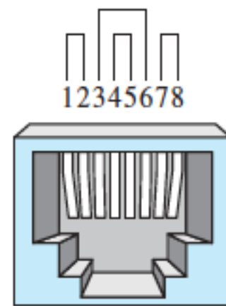
RJ-45 Female
