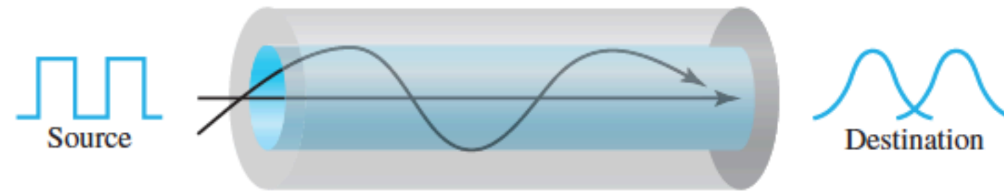
b. Multimode, graded index
