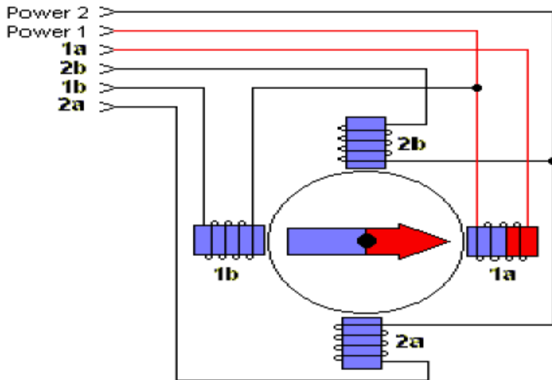
Conceptual Model of Unipolar Stepper Motor
