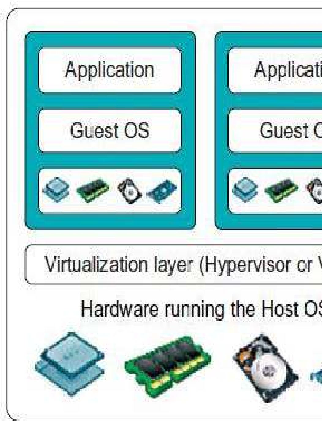
(b) After virtualization
