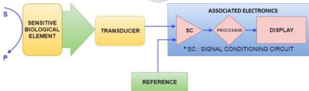
Fig -1: Schematic diagram showing main components of a biosensor
