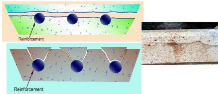
Fig.6: Concrete cracking due corrosion of reinforcement
