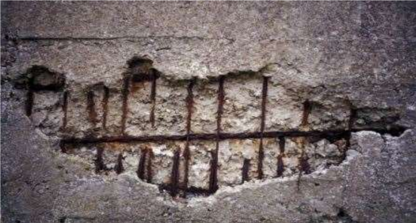
Fig 11: Corrosion of Steel in Concrete
