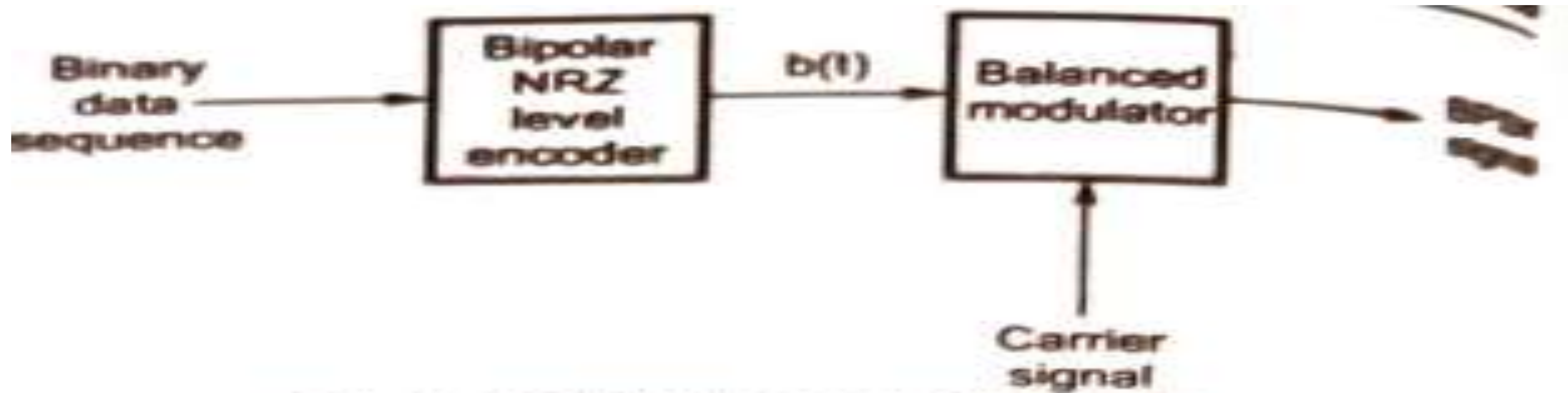
Fig. 4.7.2 BPSK generation scheme
