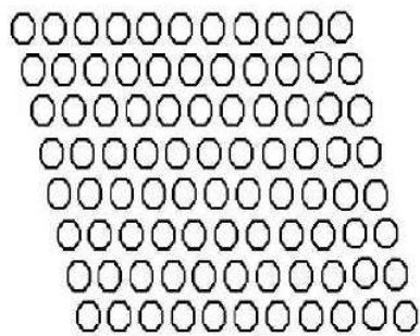
Undeformed Crystal
