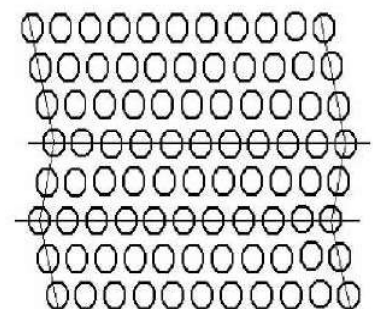
After Twinning
