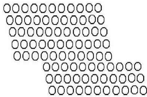
After Slip
