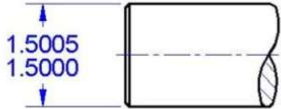
Limit Dimension
