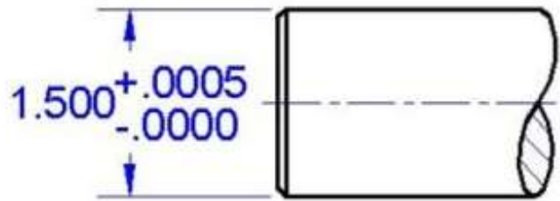
Unilateral
