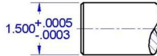
Bilateral-Unequal
